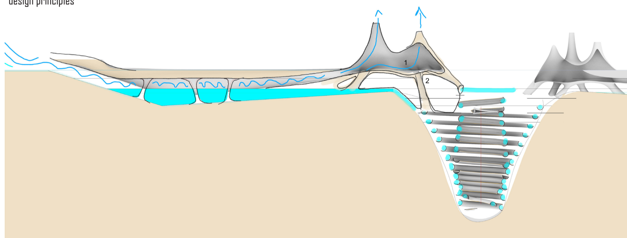
section Diagram of the passive design principles
