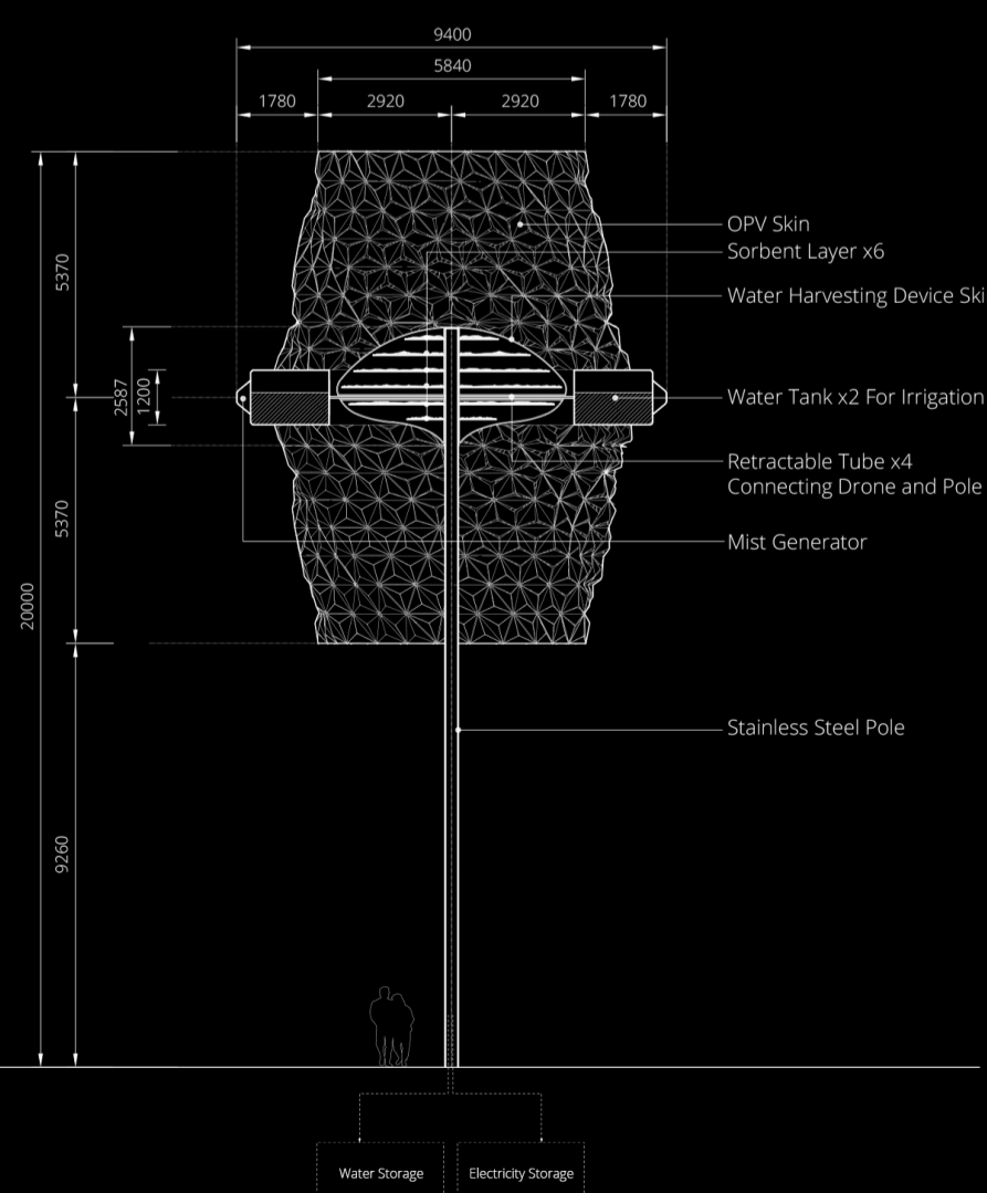
B-B Section
