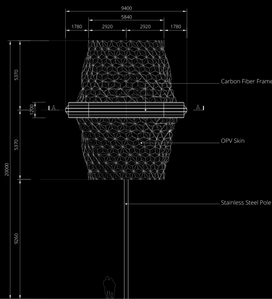
Installation Elevation
