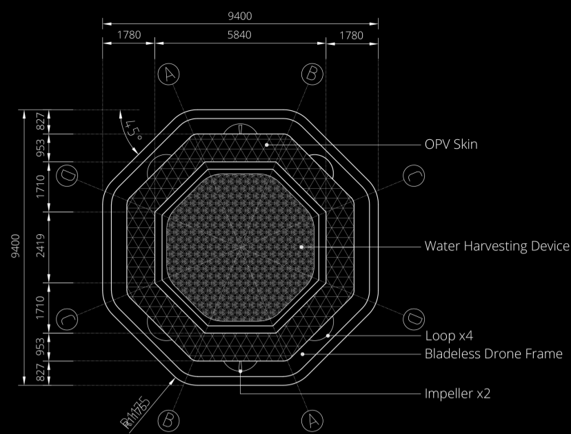
Installation Plan
