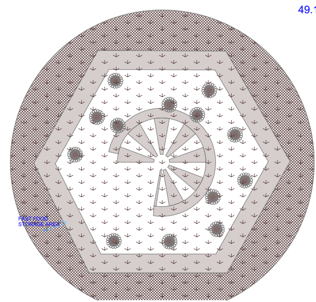
2. Story FOOD STORE LEVEL 1:100
