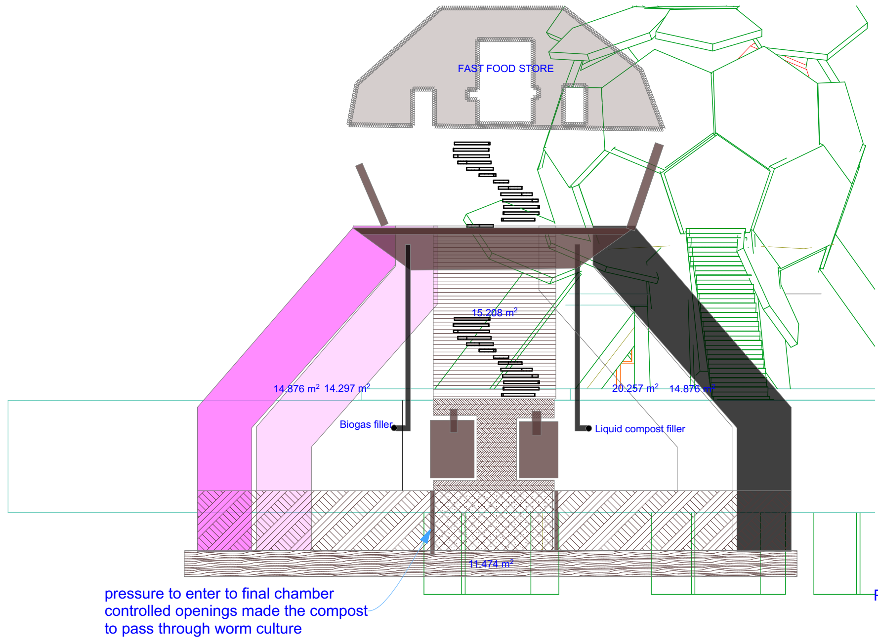
S-09 Building Section 1:100
