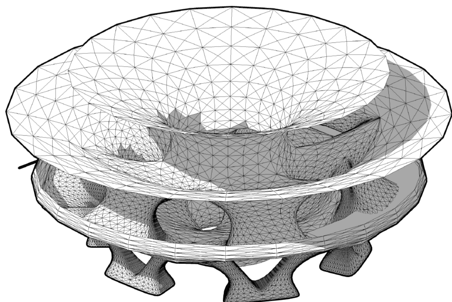
Main pavilion structure
