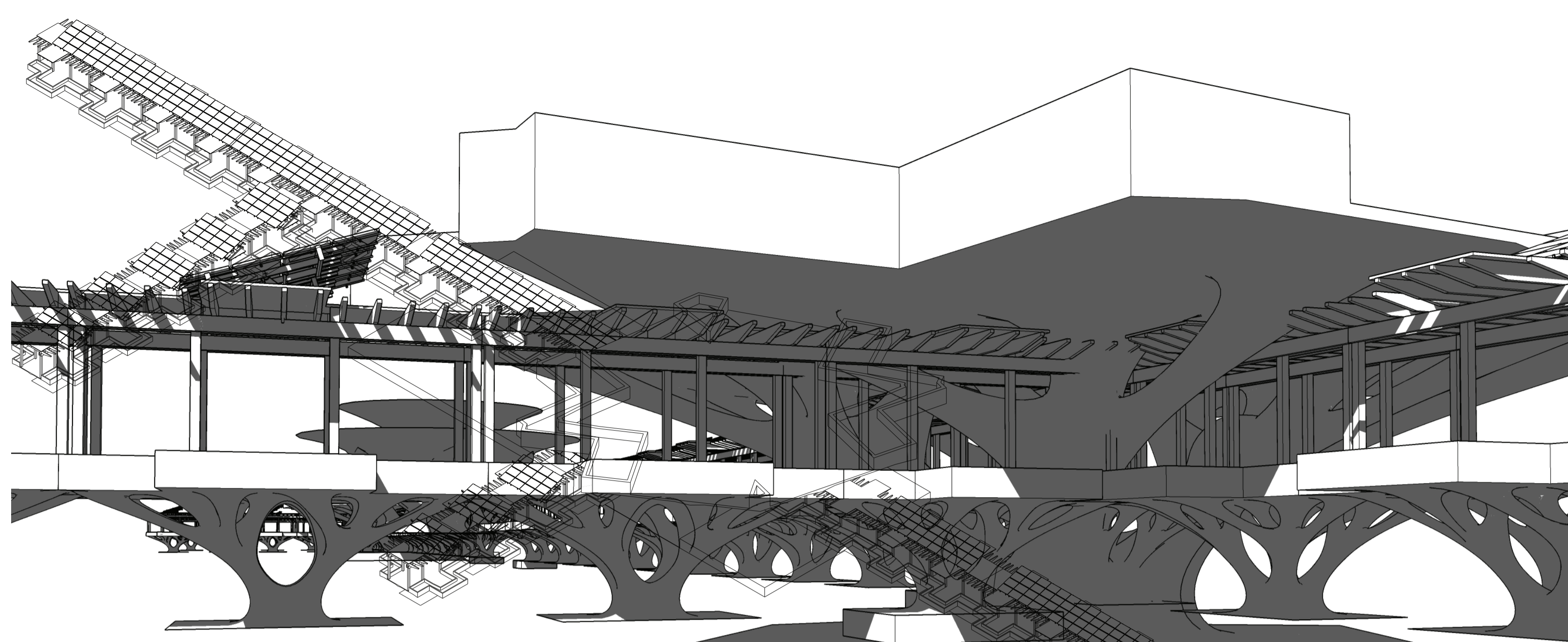
View showing the structure of the photovoltaic panels sitting on the walkway.
