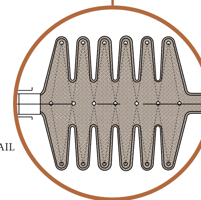
SOLAR SHADE SYSTEM DETAIL
