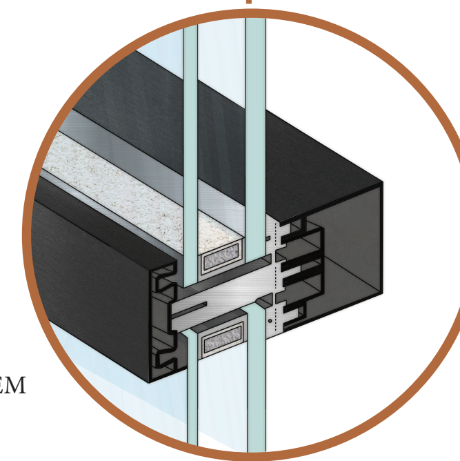
INSULATED SOLAR GLASS DETAIL
