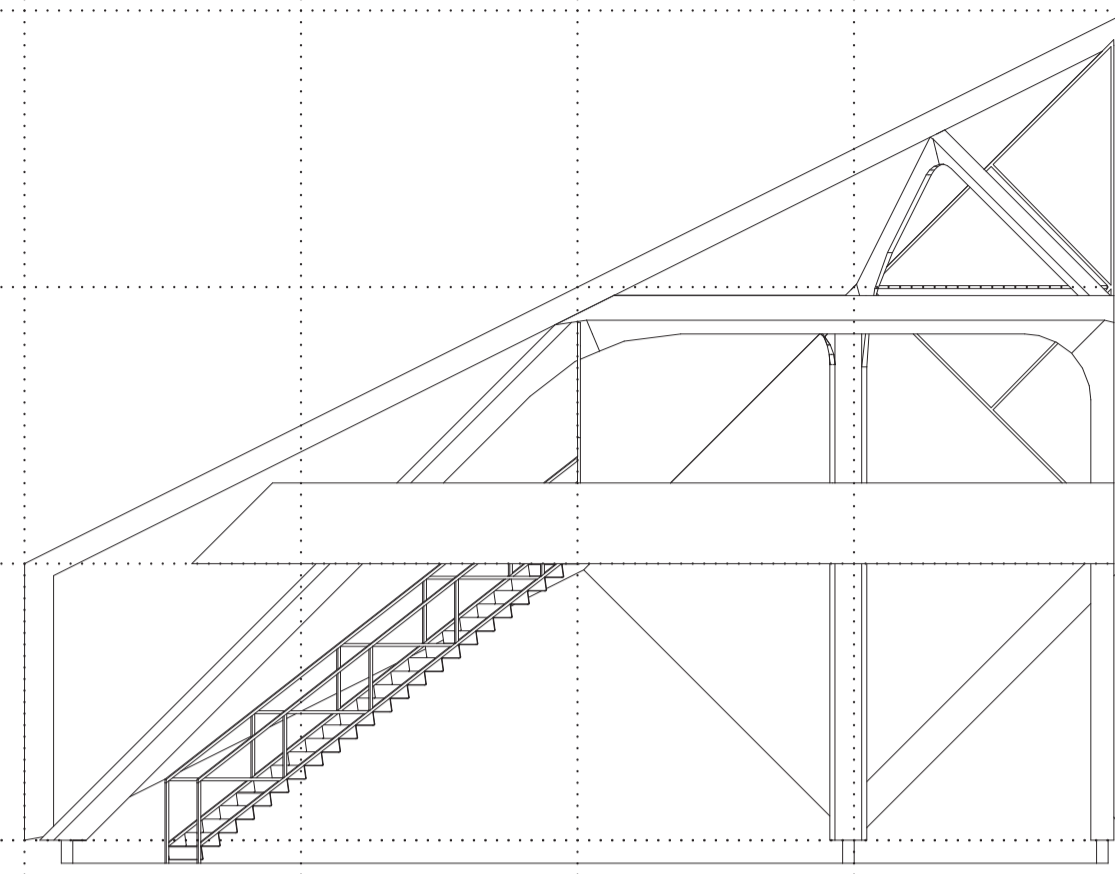
LONGITUDINAL SECTION 1/8 = 1-0
