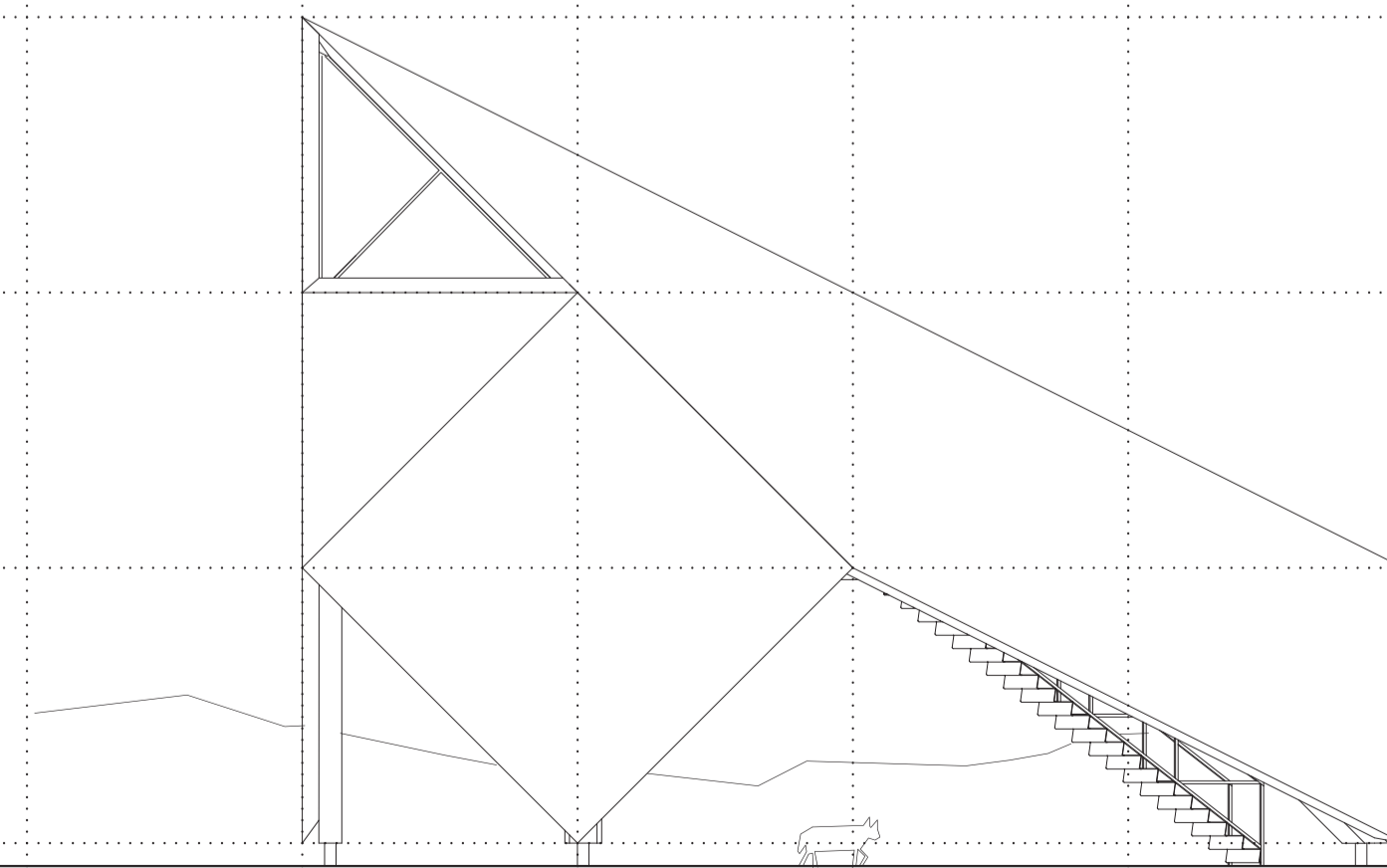
NORTH ELEVATION
