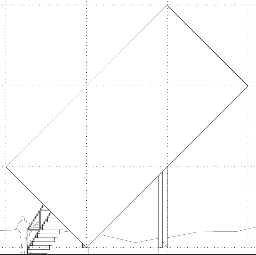
EAST ELEVATION
