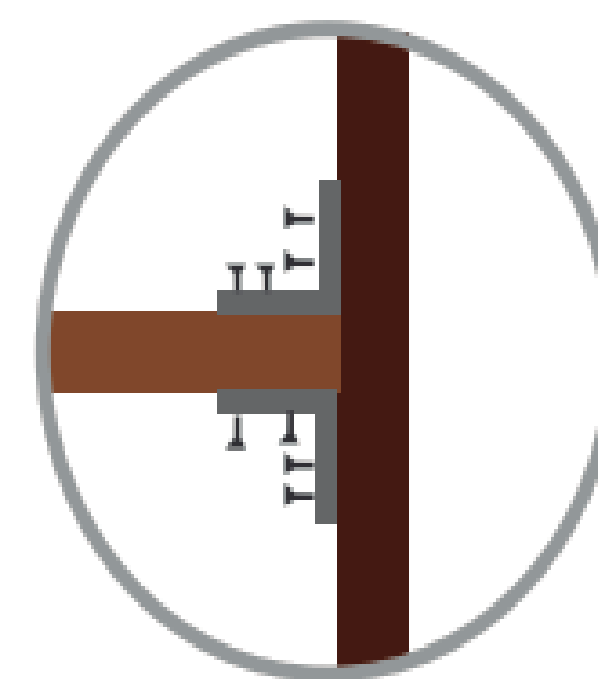
(B) Wood girder
