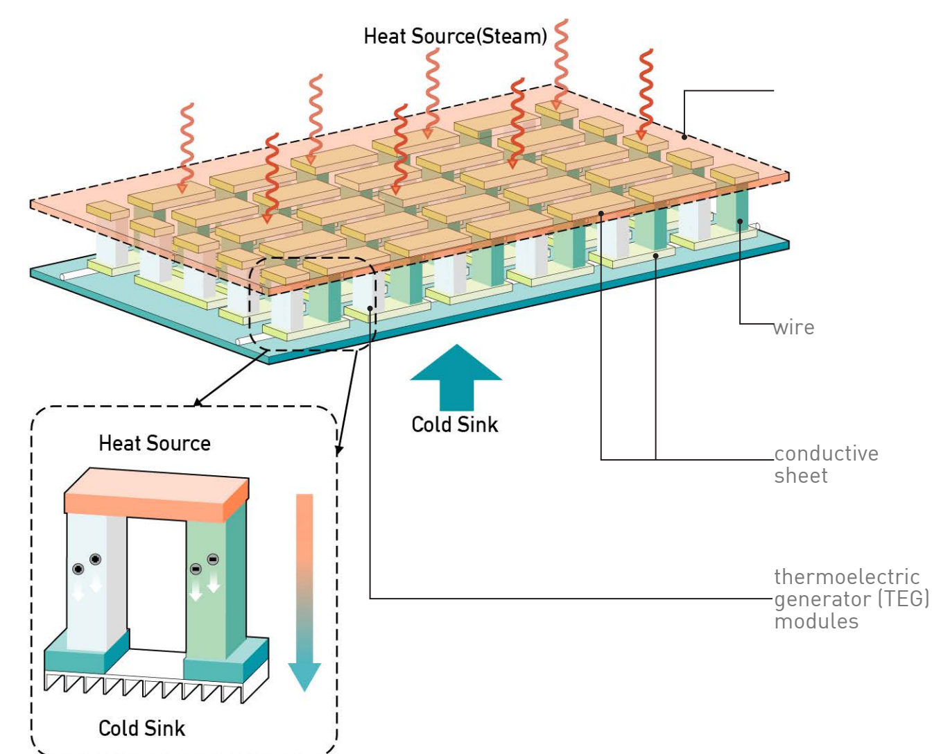
POWER GENERATION SYSTEM
