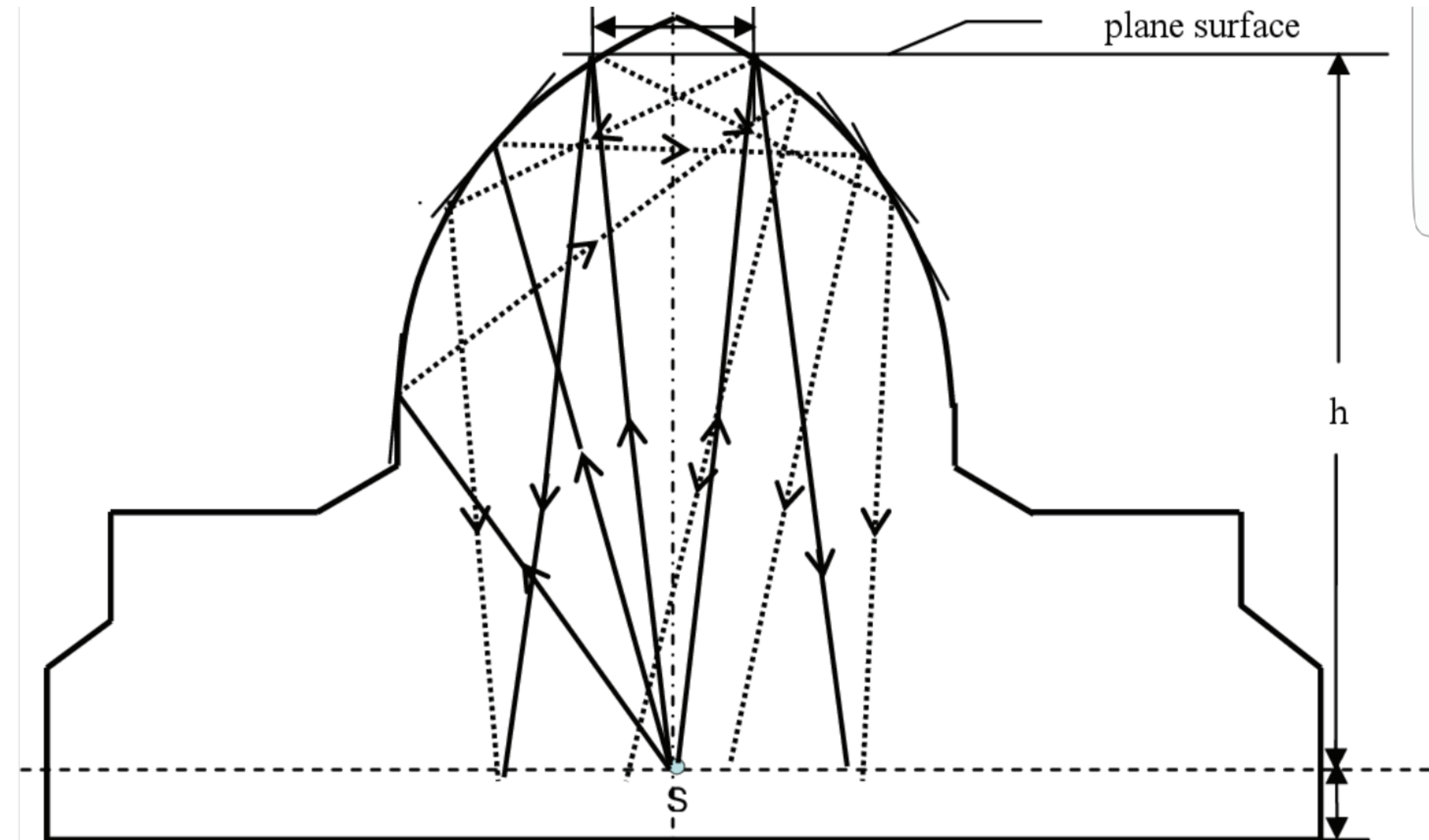
Figure 4.24. Geometrical analysis of model 4 (model 1 with an onion-shaped dome).
