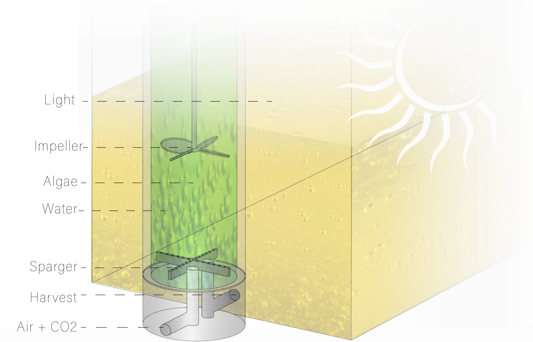
Algal Photobioreactor System
