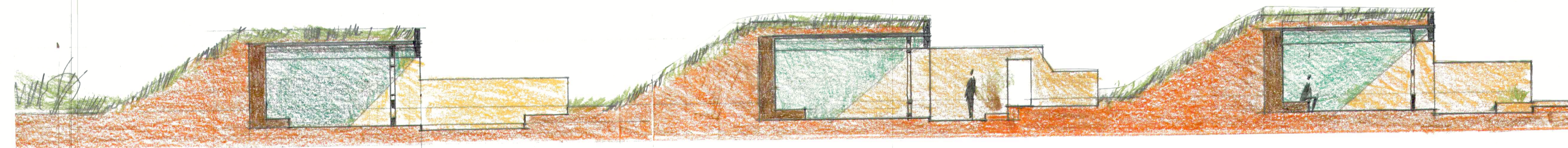
EARTH SHELTER: SECTION LOOKING EAST
