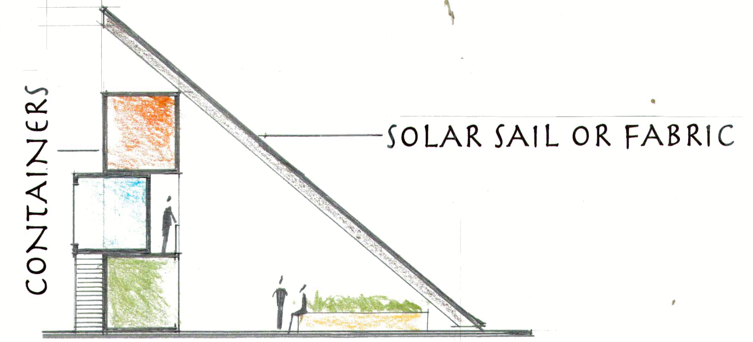
SOLAR SPINE: SECTION LOOKING EAST
