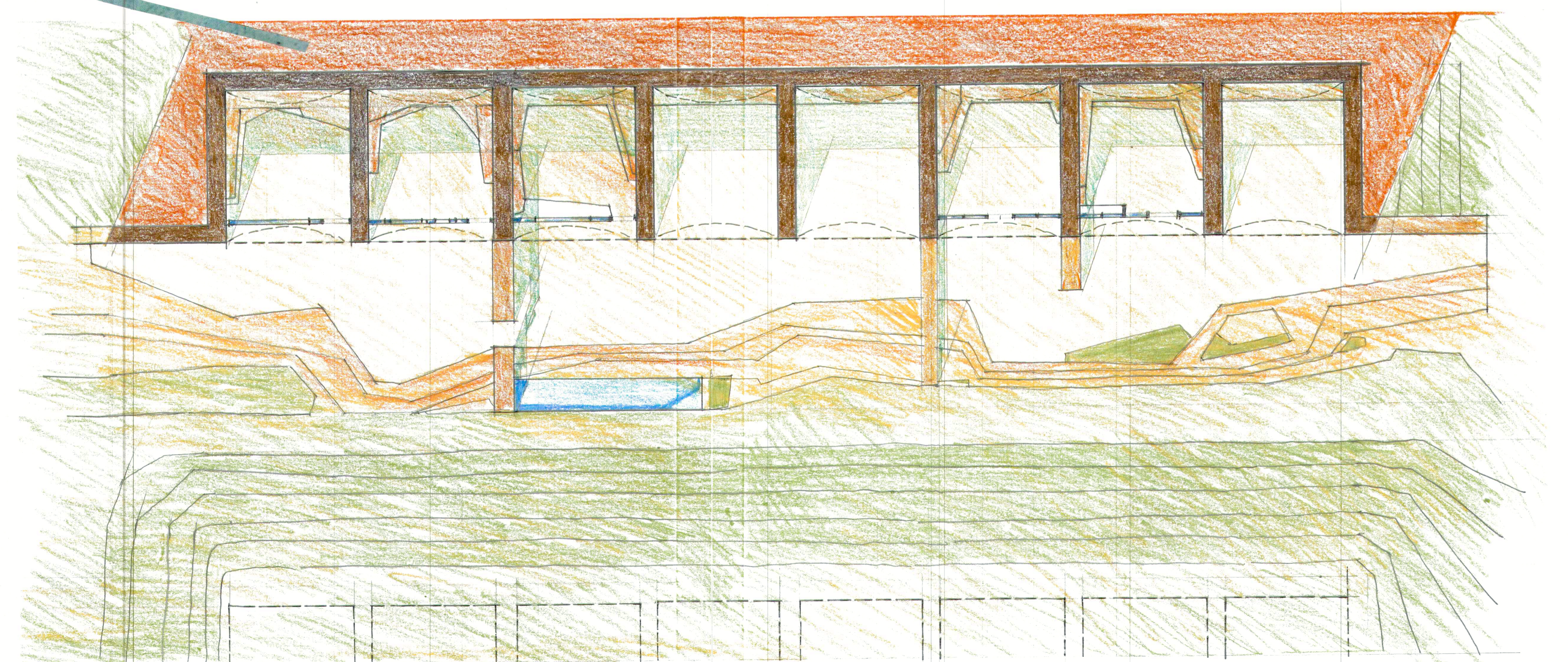
EARTH SHELTER: PLAN
