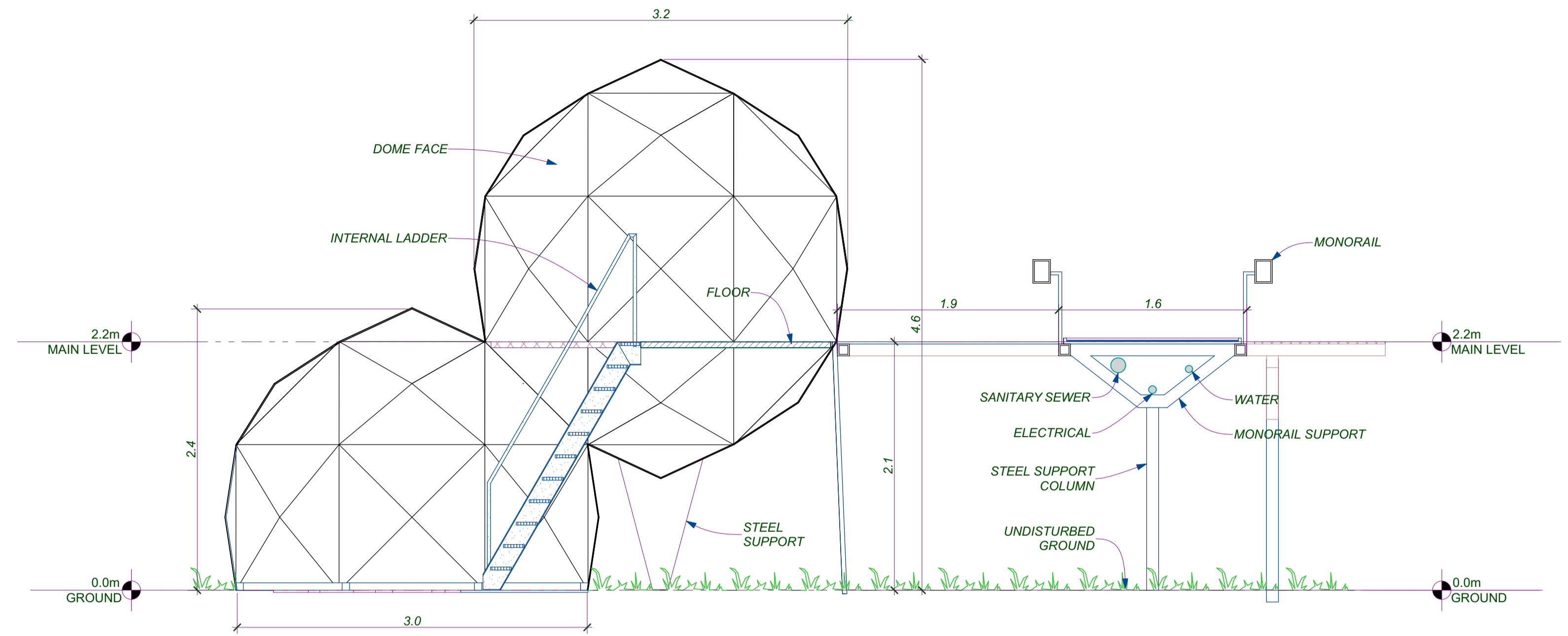
PROPOSED HONORARIUM DUPLEX and TRACK PROTOTYPE
