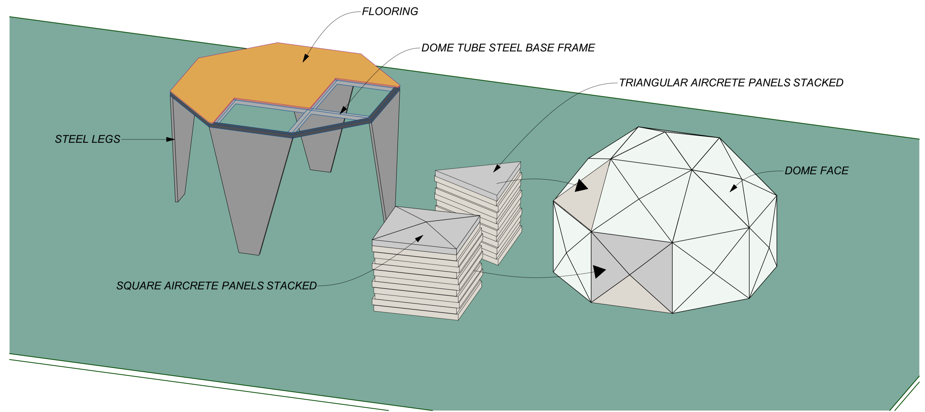
PREFABRICATED PANEL METHOD of CONSTRUCTION
