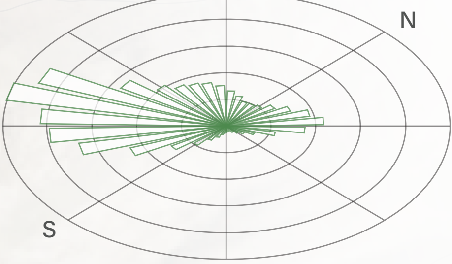
South Fly Ranch Wind Rose
