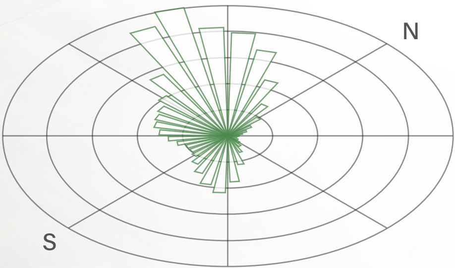
North Fly Ranch Wind Rose
