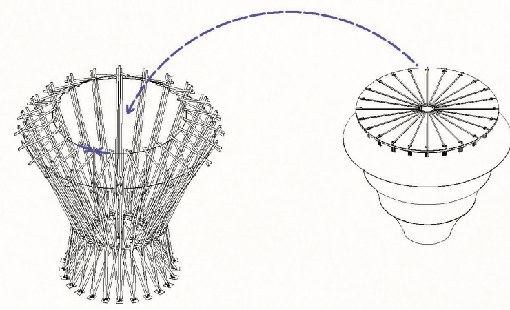
5. Insertion of fog catcher and roof elements into the main structure
