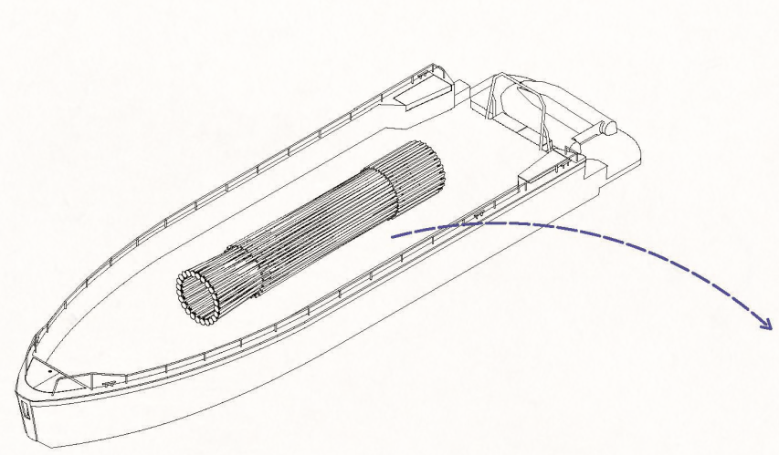
1. Prefabricated bamboo structures are packed and transported to the site by boat (size b: 4 x 14 m)
