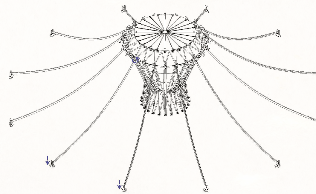
6. Assembly of secondary structural components for solar panel
