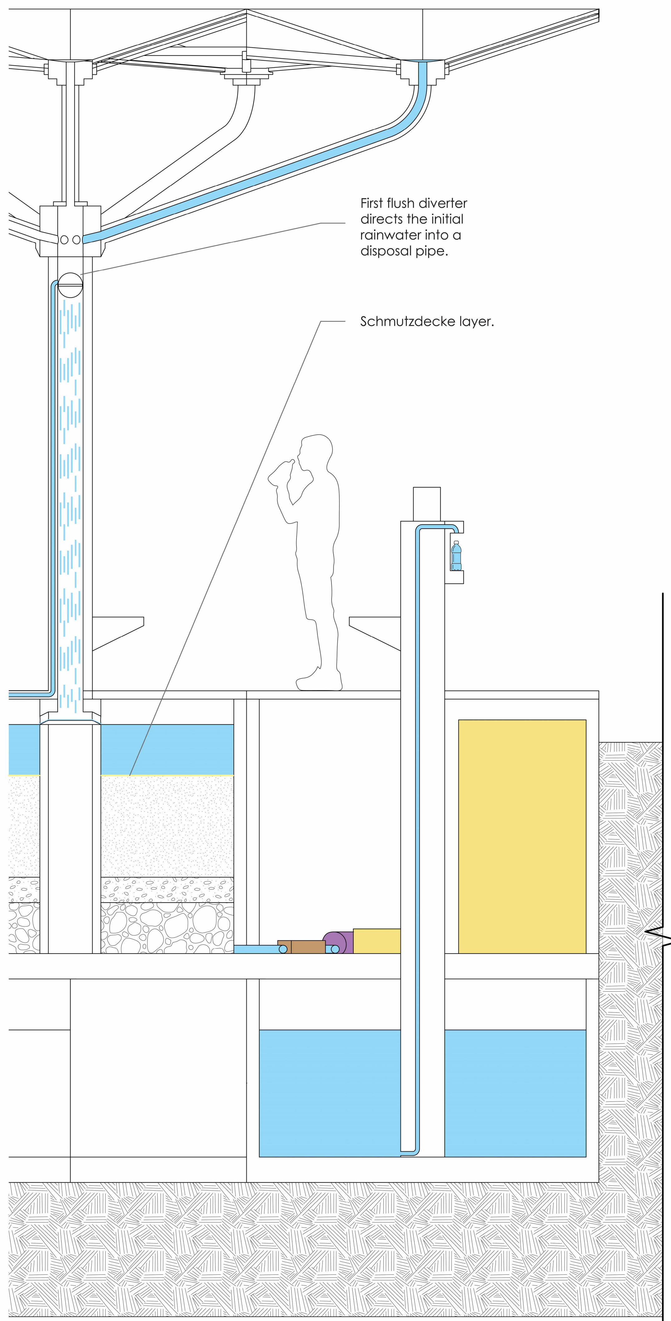
Section of Module & Water Bottle Filling Station
