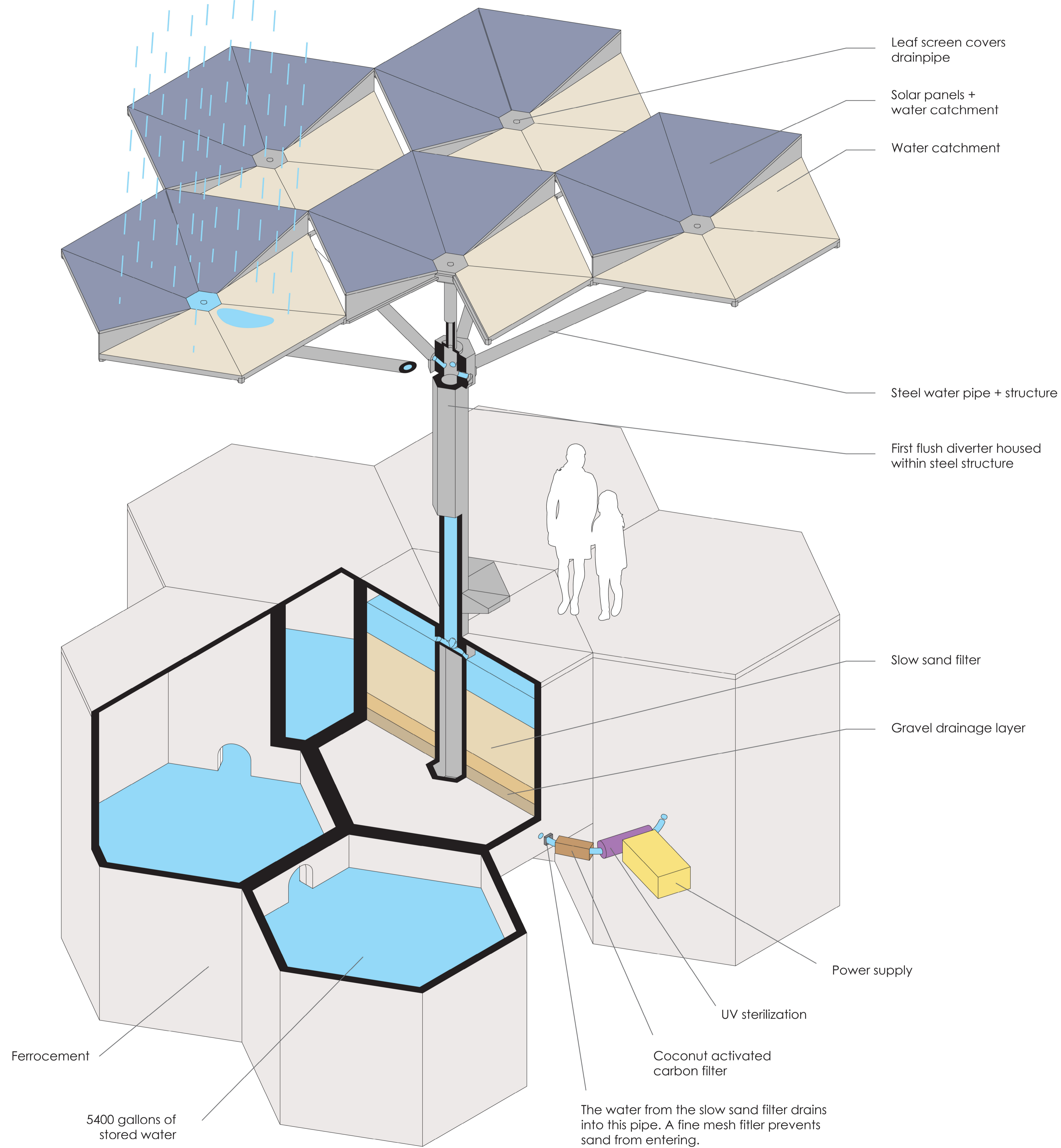
Exploded Axon of Module
