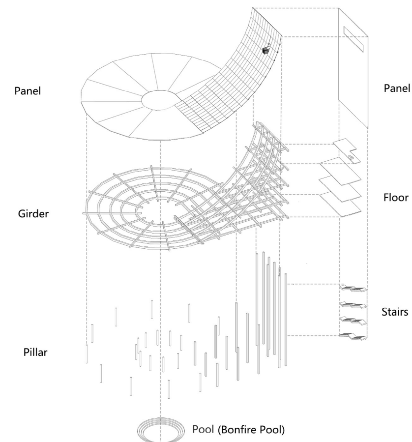
Exploded view
