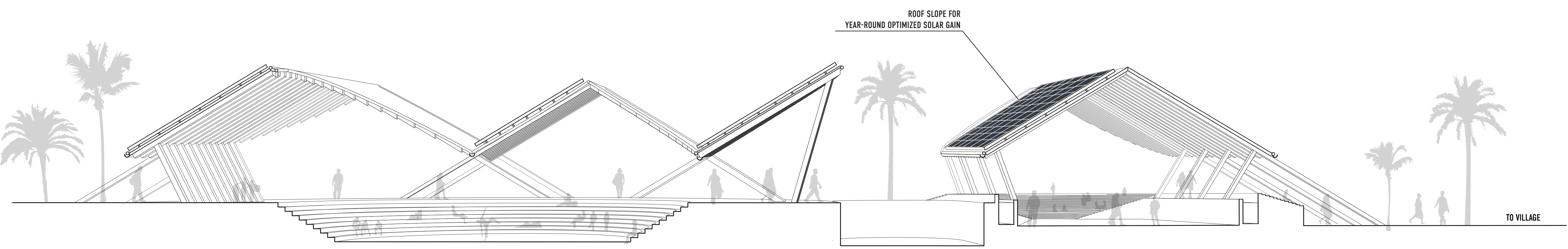
EAST ELEVATION
