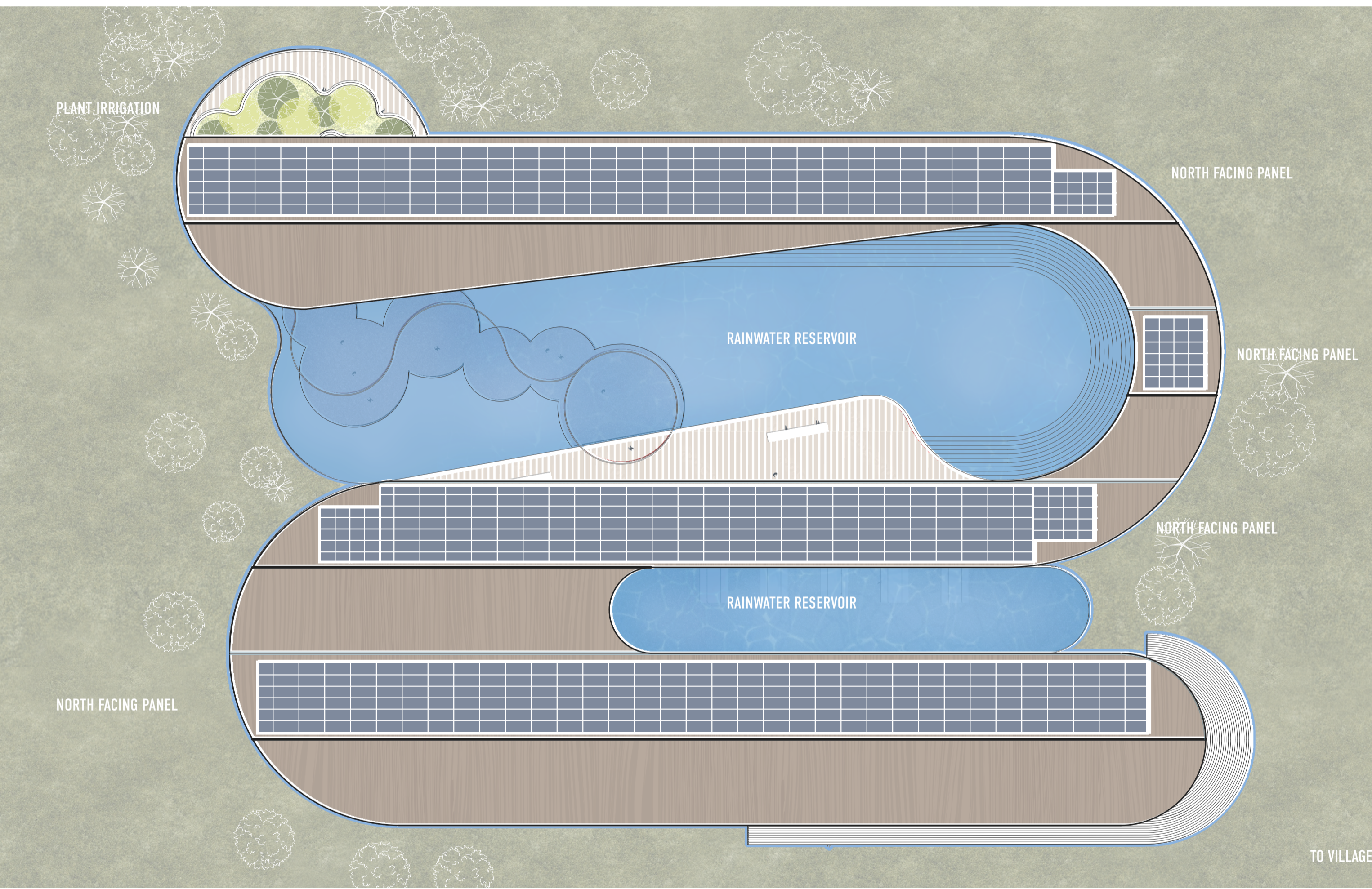
ROOF PLAN
