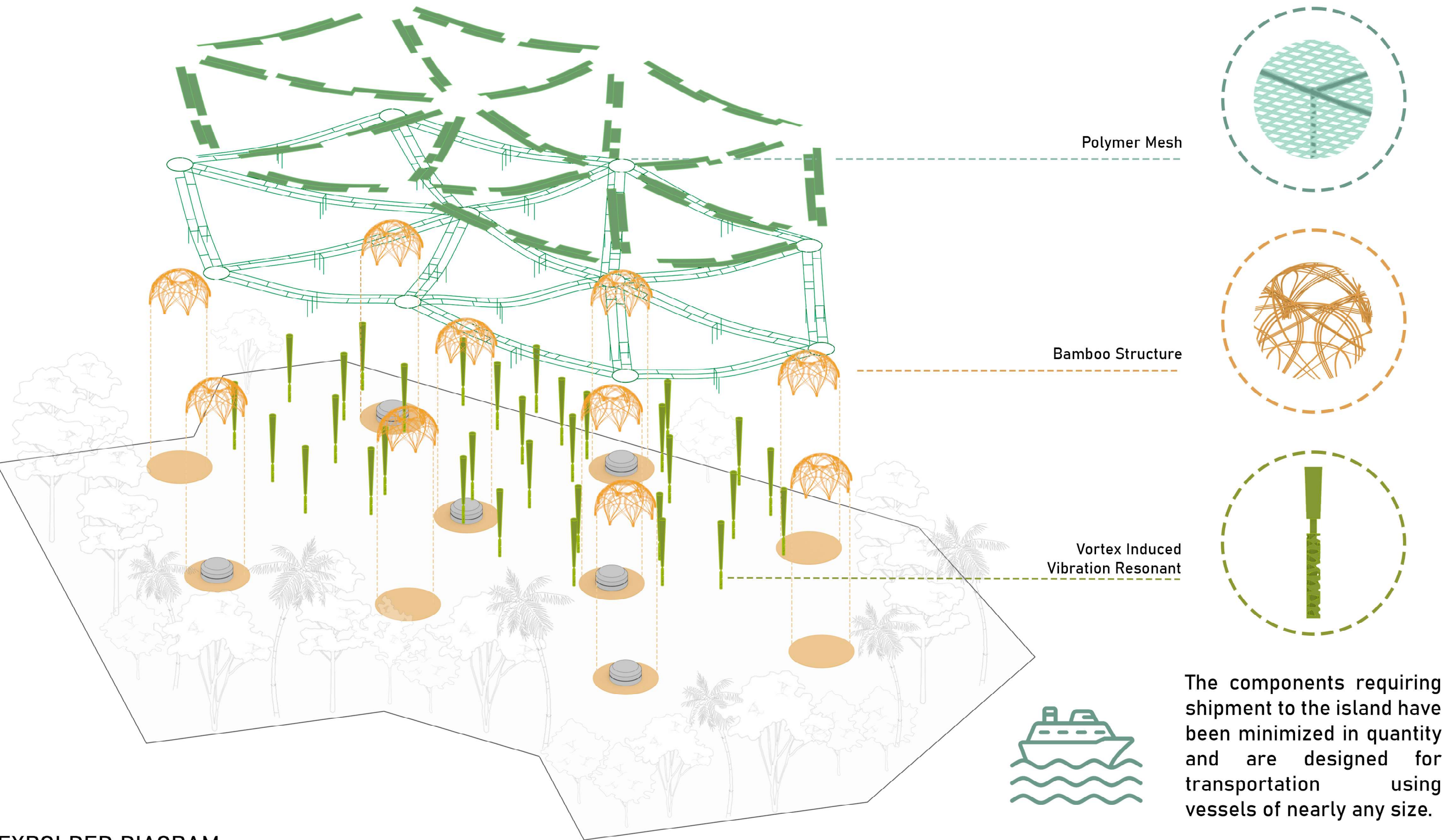
EXPLODED DIAGRAM
