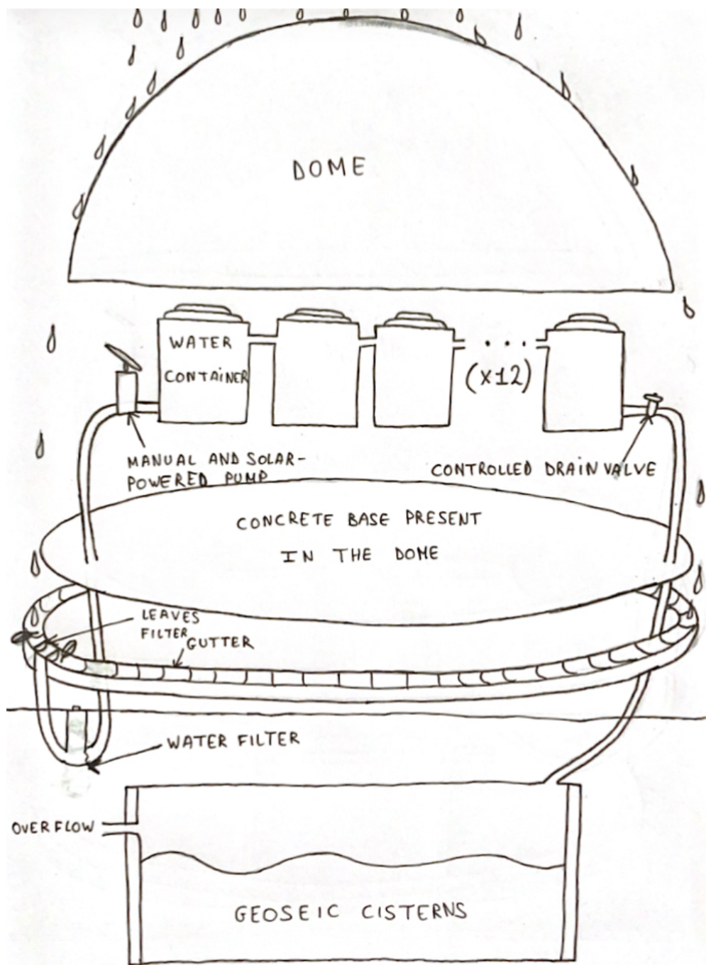
EXPLODED VIEW OF THE RAINWATER HARVESTING SYSTEM
