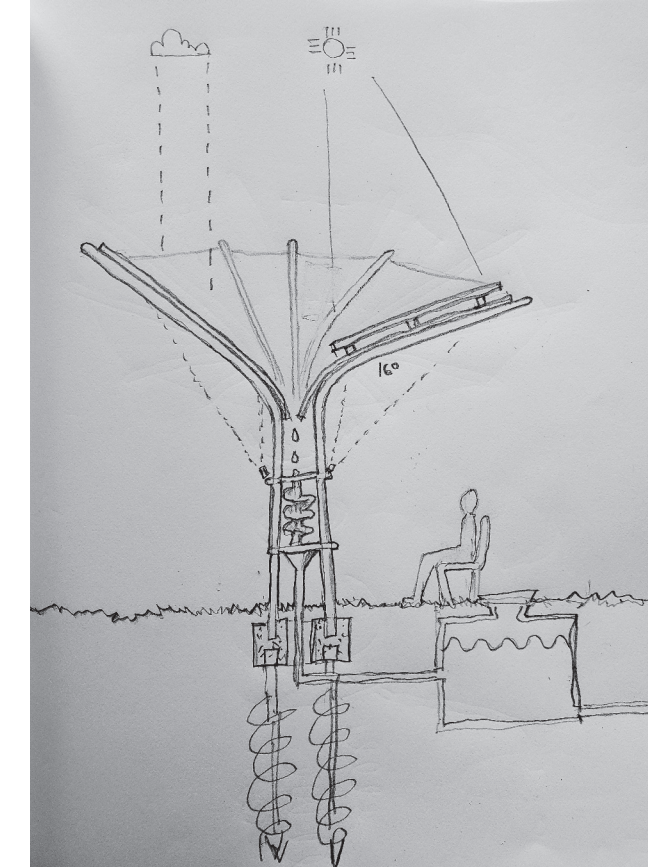
INITIAL SUN & RAIN COLUMN DIAGRAM
