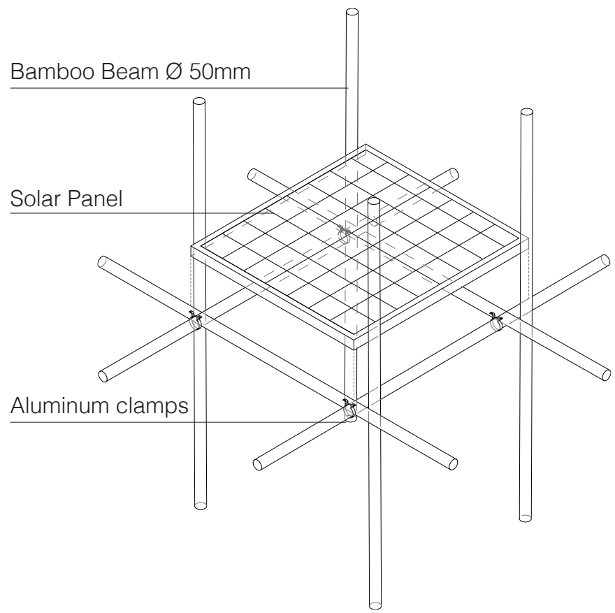
Detailed Section 1:10
