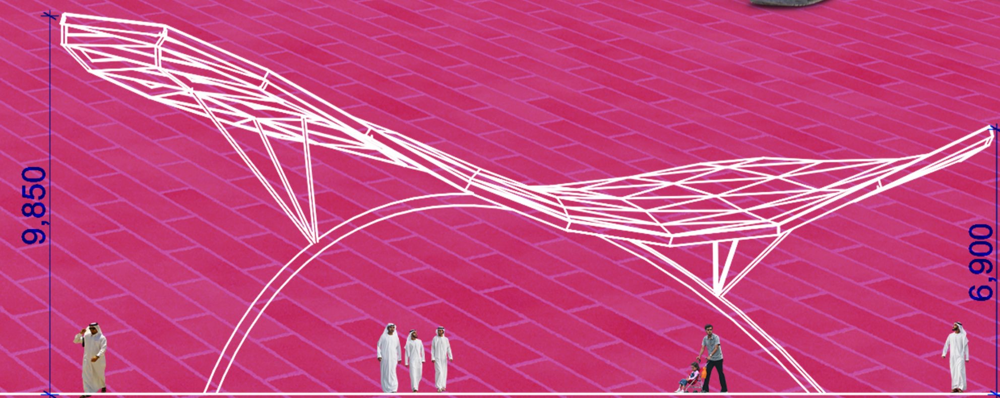
Side view of the photovoltaic butterfly sculpture.
