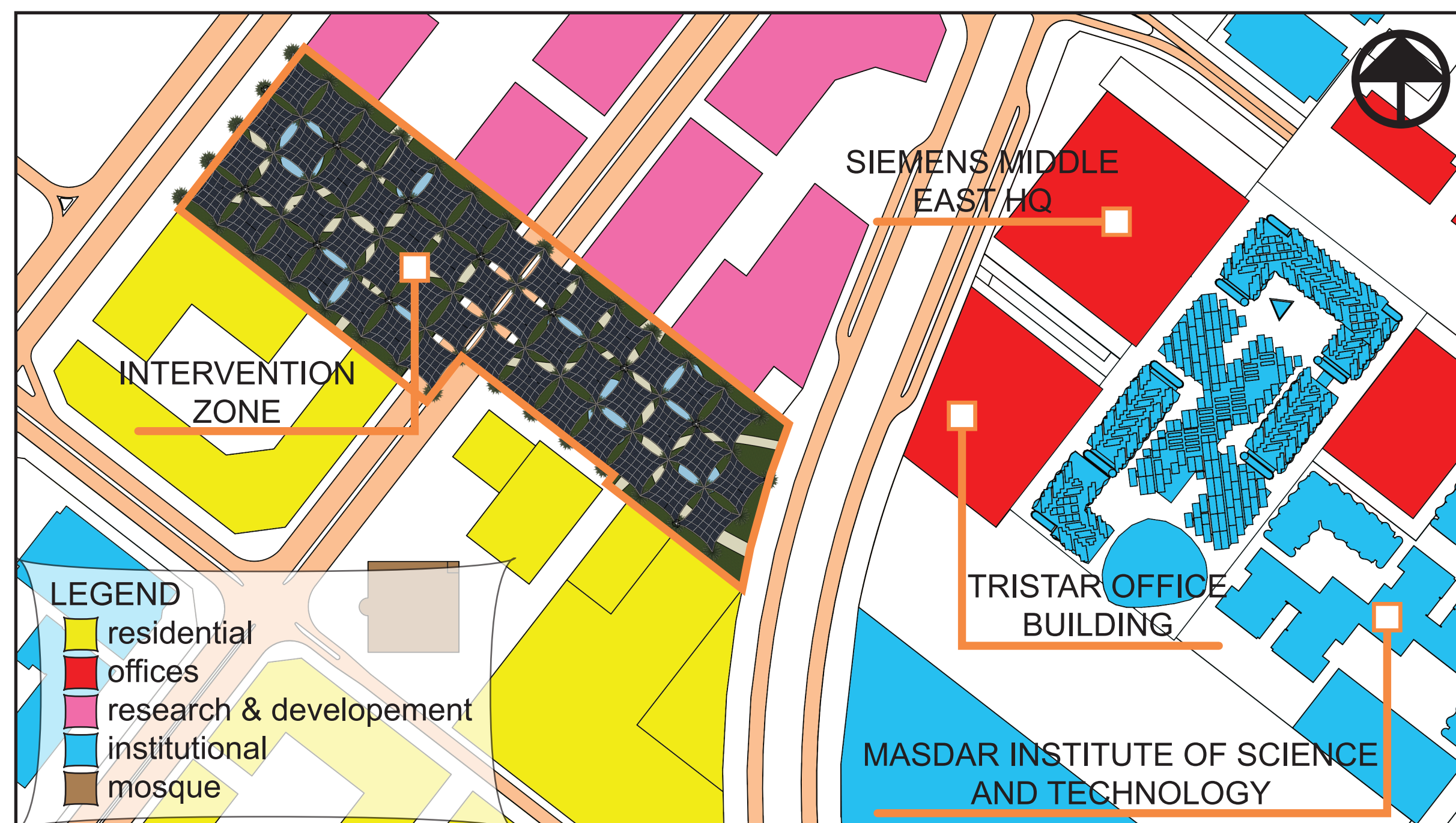
MASTERPLAN SCALE 1/2000
