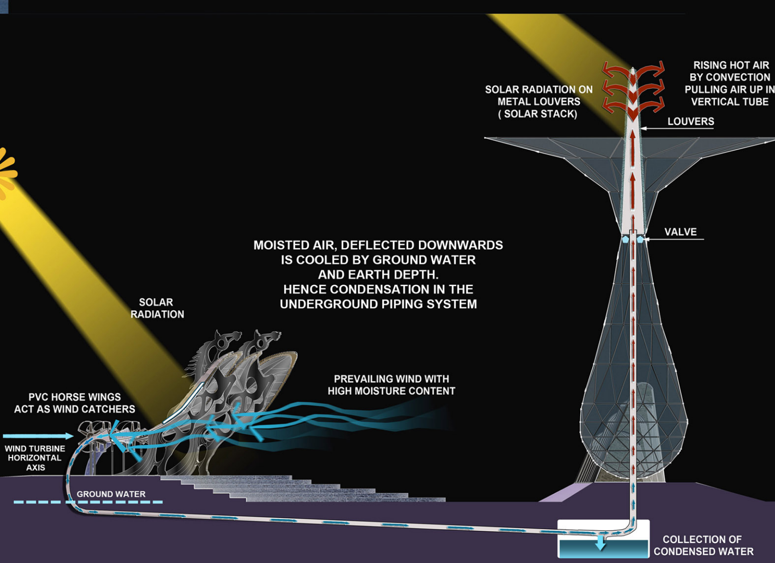
1ST SYSTEM... FOR PRODUCING POTABLE WATER FROM ATMOSPHERE
