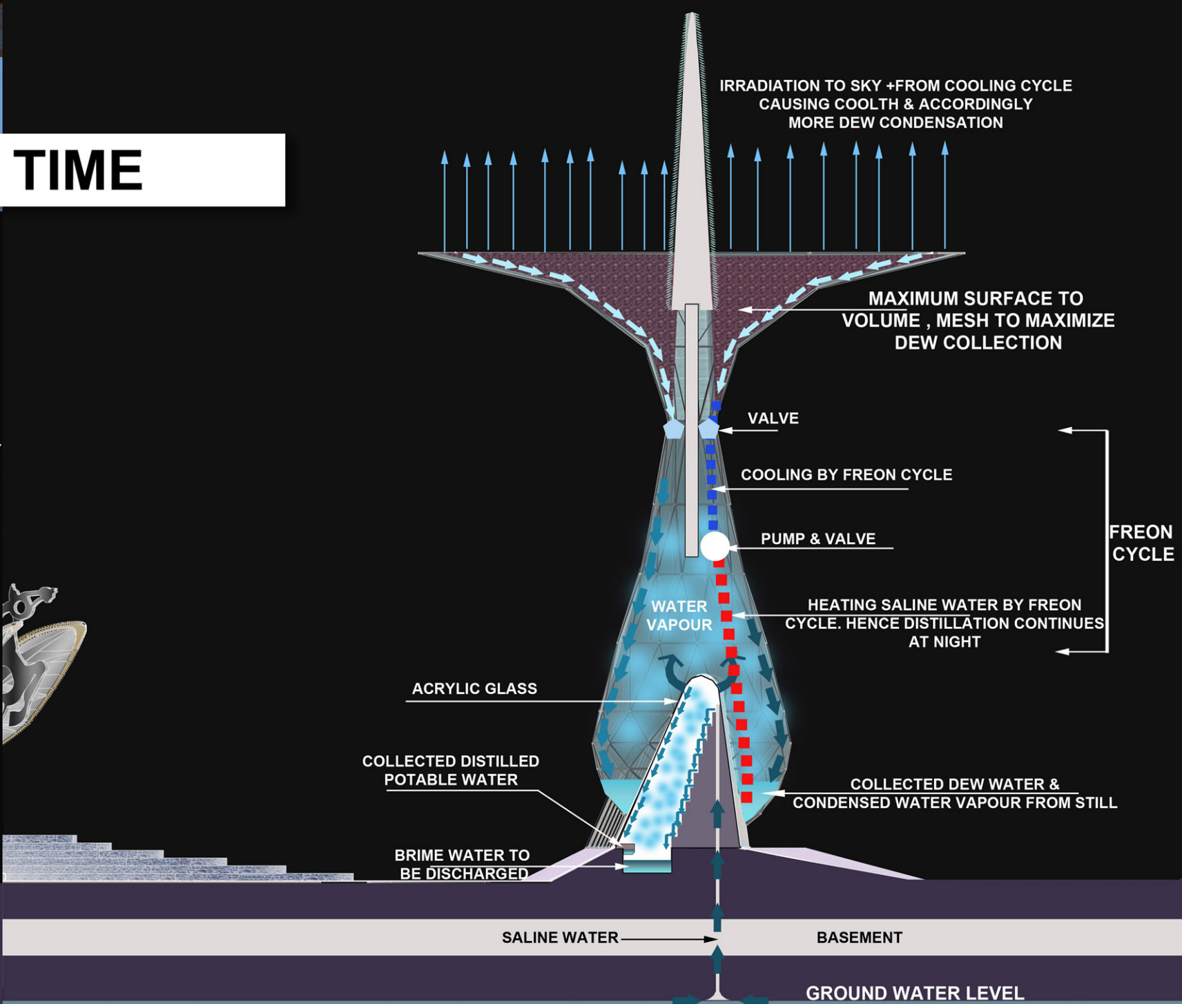
4TH SYSTEM.. FOR PRODUCING POTABLE WATER THROUGH FREON CYCLE COOLING DEW MESH & HEATING GROUND WATER BEFORE ENTERING SOLAR STILL + CONTINUATION OF UNDERGROUND CONDENSATION
