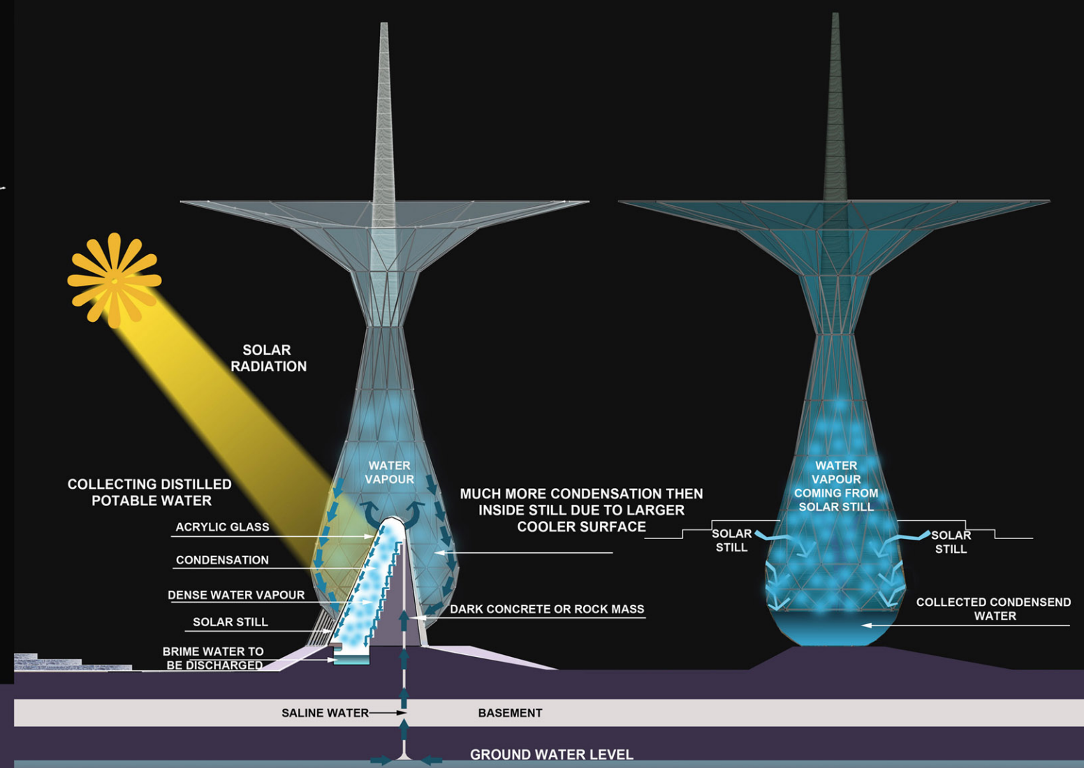
2ND SYSTEM.. FOR PRODUCING POTABLE WATER-FROM SOLAR DISTILLATION
