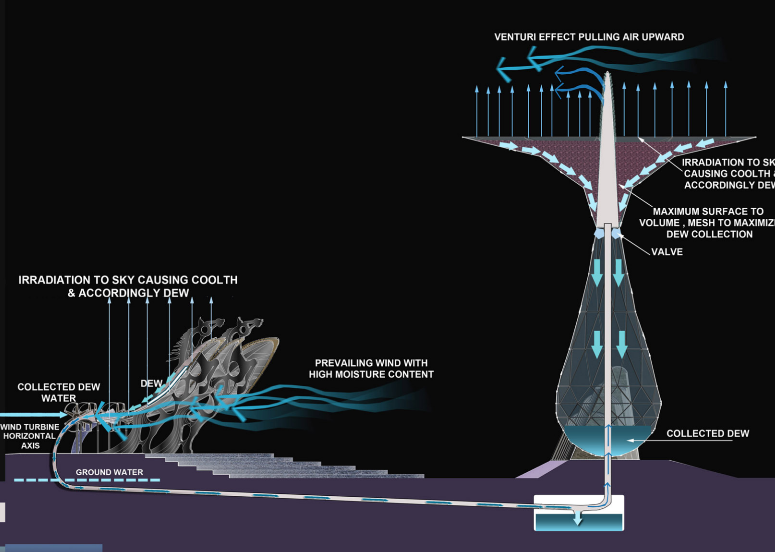
3RD SYSTEM.. FOR PRODUCING POTABLE WATER BY DEW COLLECTION +CONTINUATION OF UNDER-GROUND CONDENSATION
