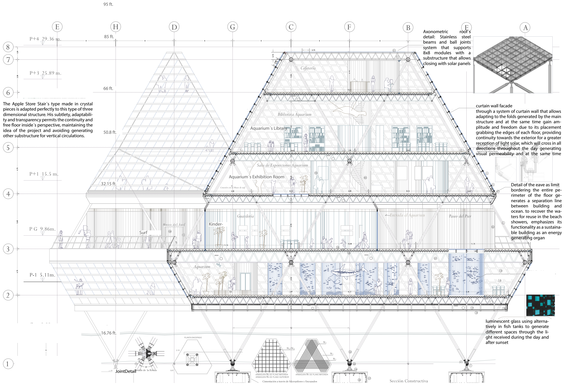
Constructive Section Scale_Aquarium
