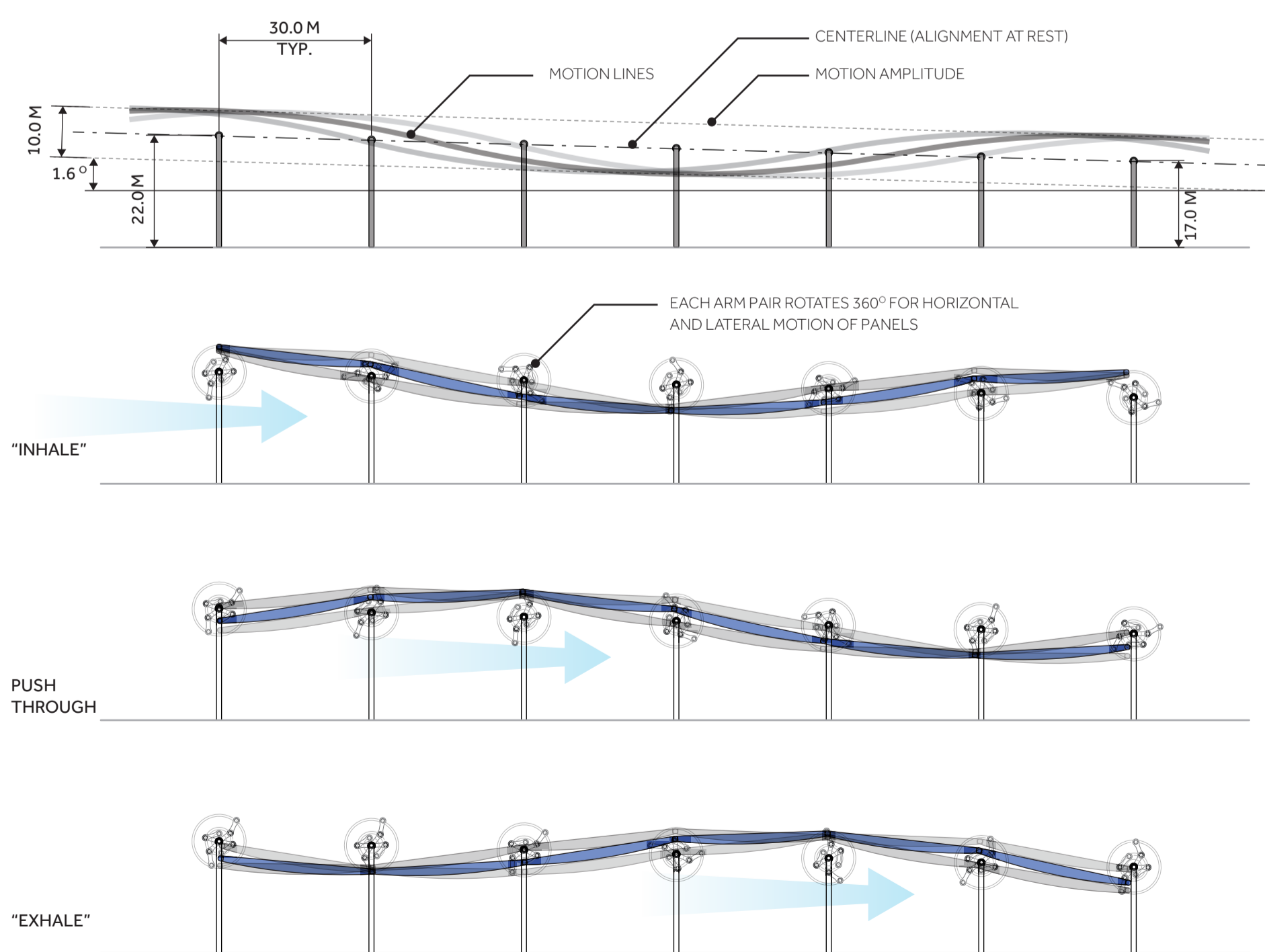
SECOND SKY MOVEMENT SECTION SCALE 1:1000
