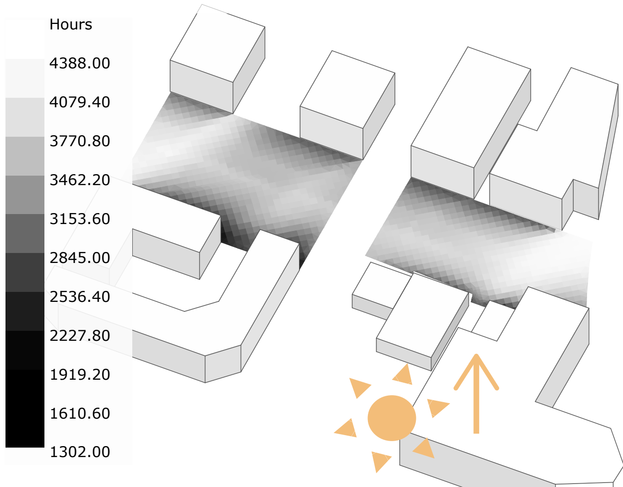
SUNLIGHT ANALYSIS - HOURS OF DIRECT SUNLIGHT / YEAR
