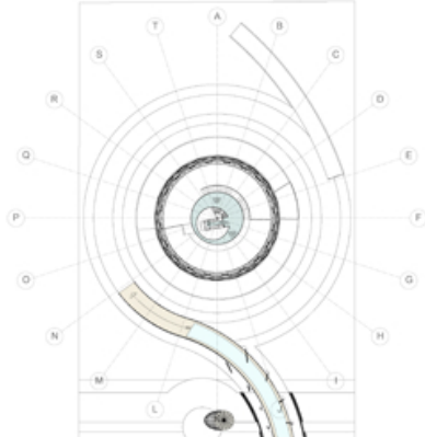
MEZZANINE FLOOR PLAN
