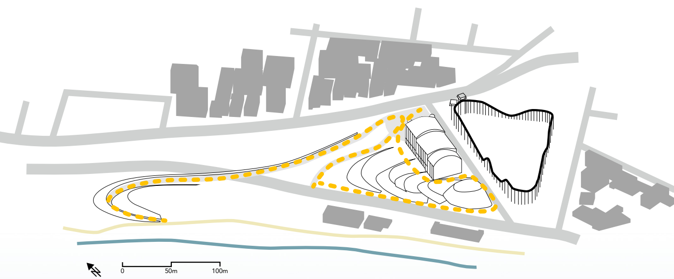
PEDESTRIAN PATHS
