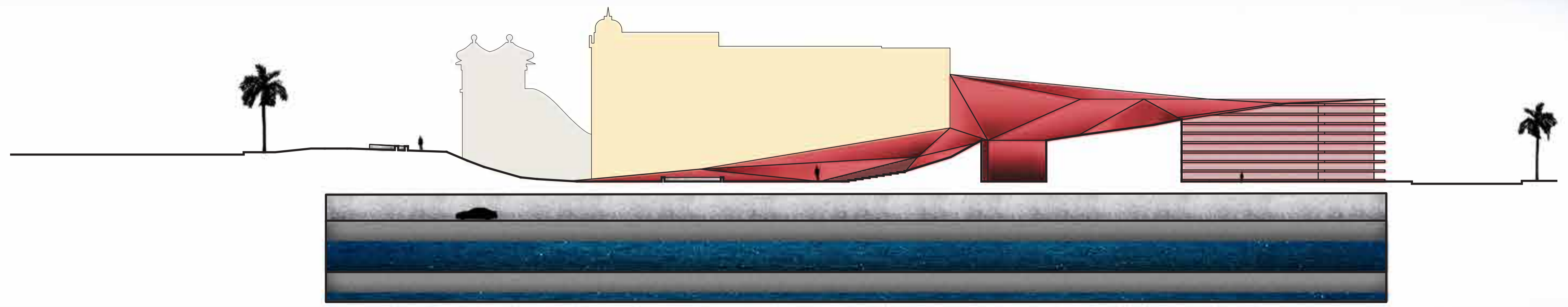
LONG SECTION 1:500
