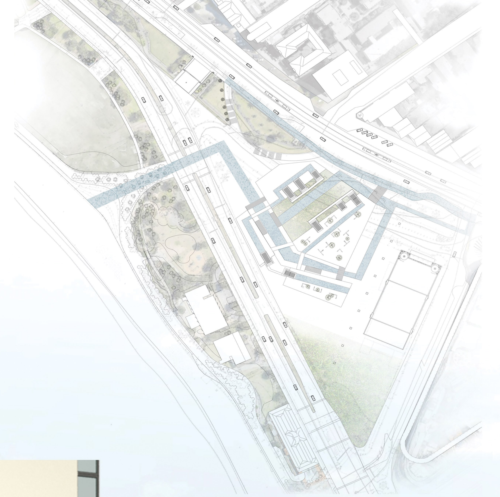
Site Plan
